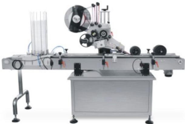
Plastic Cover Plane Labeling Machine
